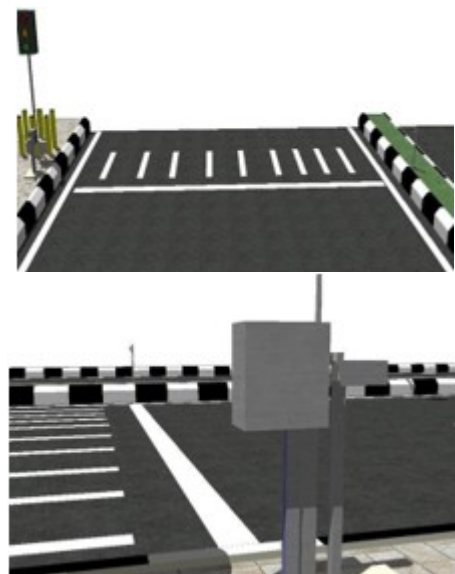
Gambar 7 Model Alat 3D
